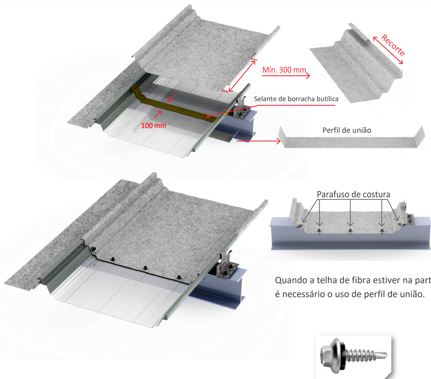
Parafuso de costura PB 1/4 – 14x7/8"
